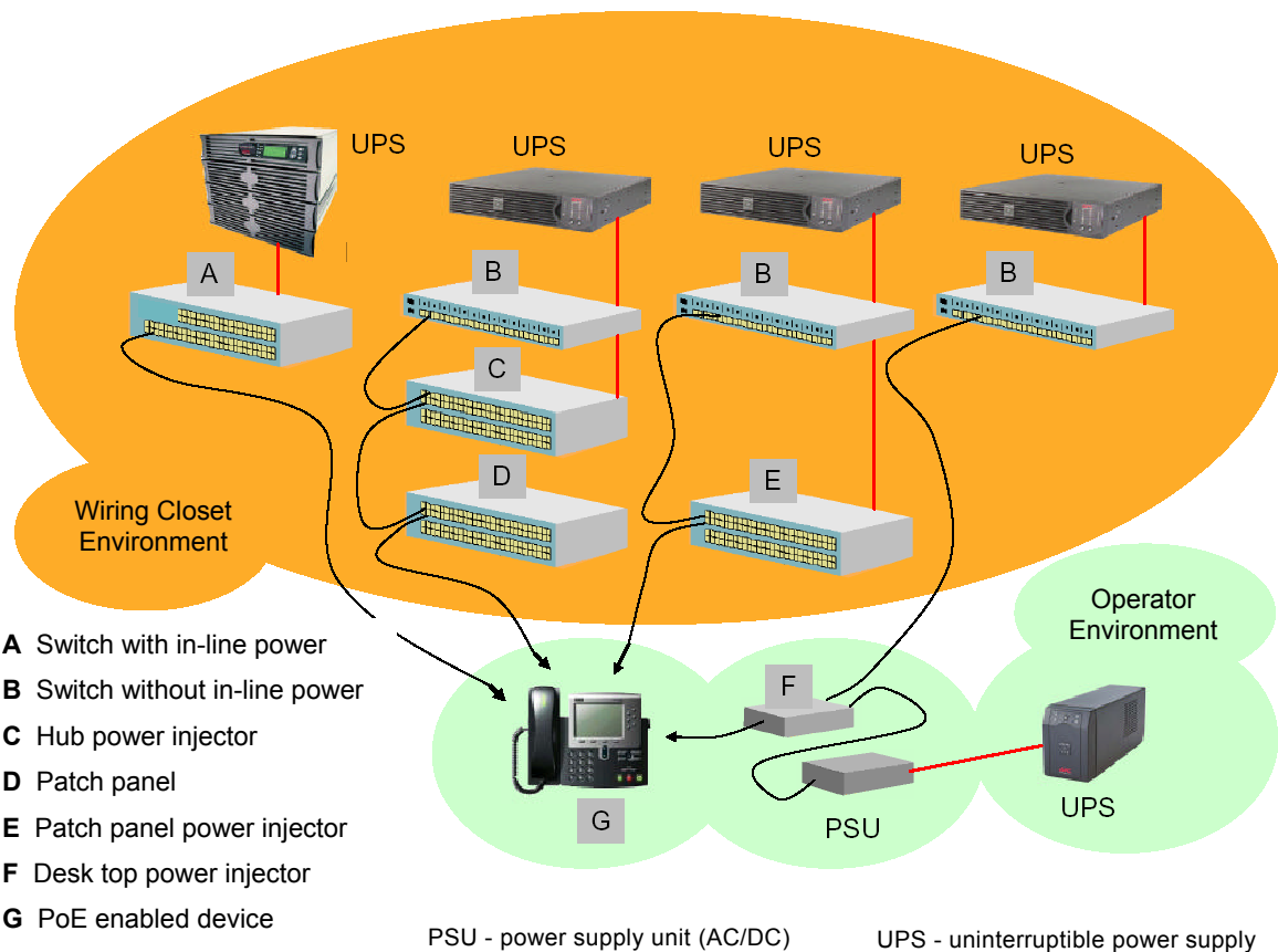
Figure 1 Typical PoE component layout
