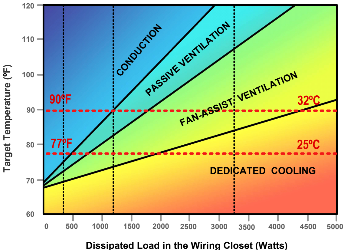
Figure 7 Wiring closet temperature versus dissipated load and associated cooling
